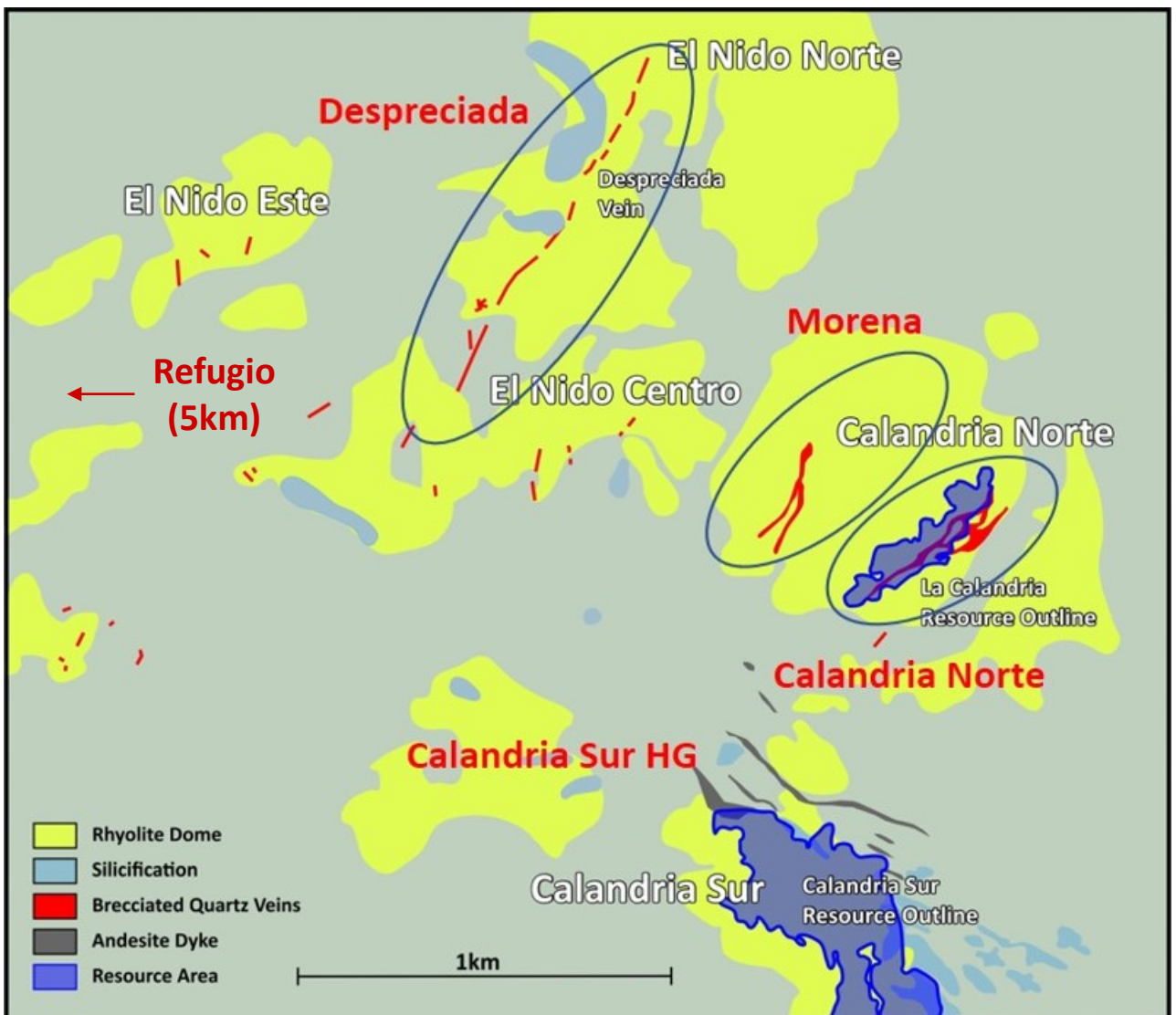
Figure 2: Las Calandrias Project – Main Targets and Mineral Resource Areas
