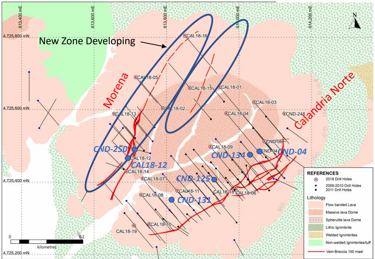
Figure 3: Las Calandrias - 2018 Drilling and Metallurgical Sample Locations
